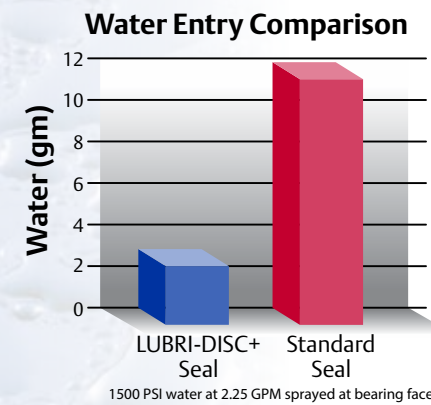
LUBRI-DISC + Seal
